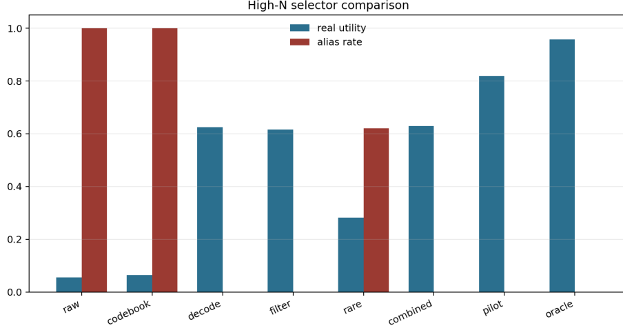
Figure 3: High-budget selector comparison. Real utility and alias rate are plotted together so repair gains cannot hide residual aliasing or oracle gaps.
