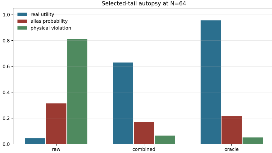
Figure 6: Selected-tail autopsy at N = 64 . Raw selection picks alias-heavy, physically invalid futures; combined repair and oracle shift the selected tail toward real utility.
