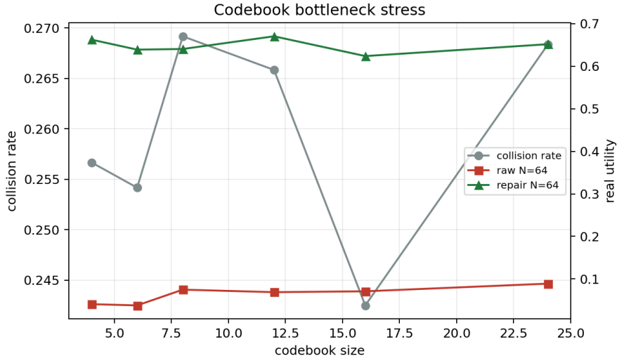
Figure 11: Codebook bottleneck curve from the original full artifact.
