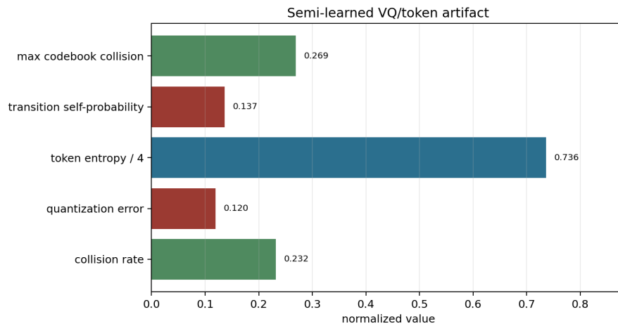
Figure 15: V3 semi-learned VQ artifact summary.
