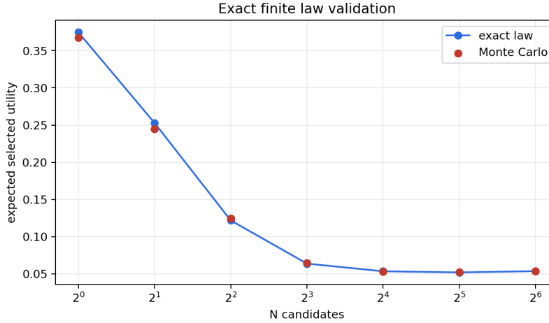
Figure 9: The finite tie-aware law predicts selected real utility for the fixed empirical token-future pool. Residuals are Monte Carlo estimation error rather than asymptotic approximation error.
