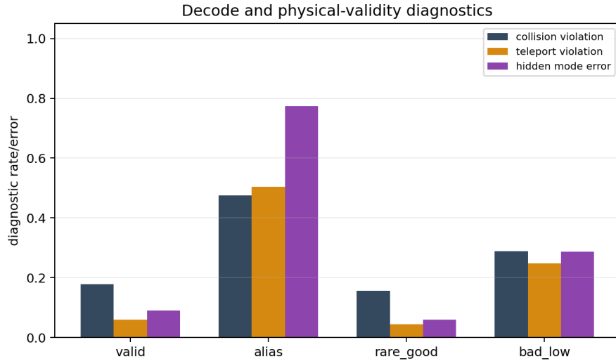
Figure 7: Decode and physical-validity diagnostics. These are the token-specific signals used to distinguish plausible token futures from valid physical futures.
