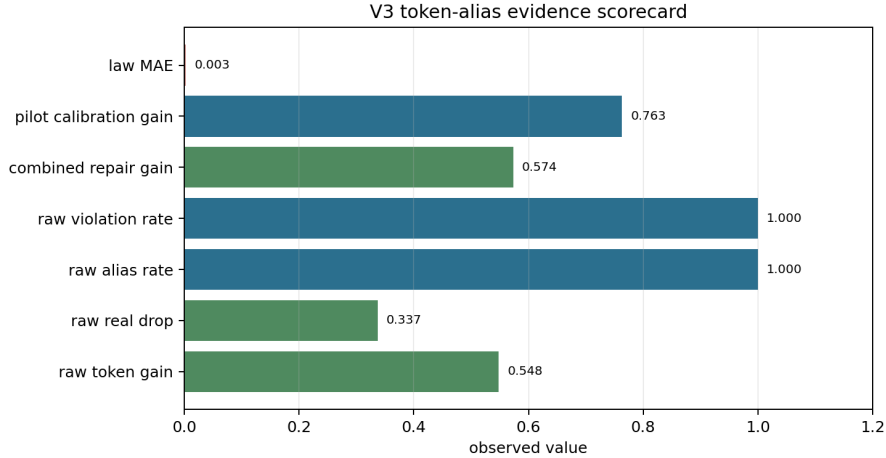
Figure 1: V3 token-alias evidence scorecard. The central pattern is token-score improvement paired with real-utility collapse, aliasing, and physical invalidity in the raw high-budget tail.
