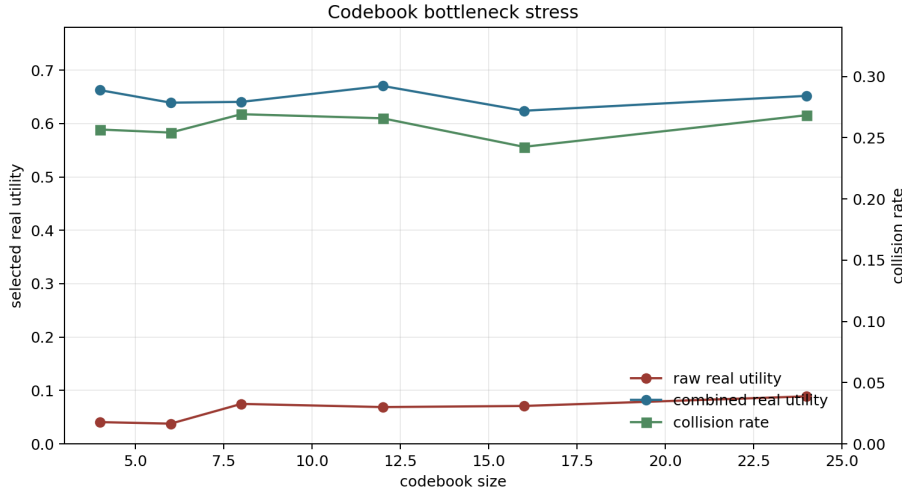
Figure 5: Codebook bottleneck stress. Increasing codebook size reduces quantization pressure but does not remove hidden-mode collision in this controlled setup.
