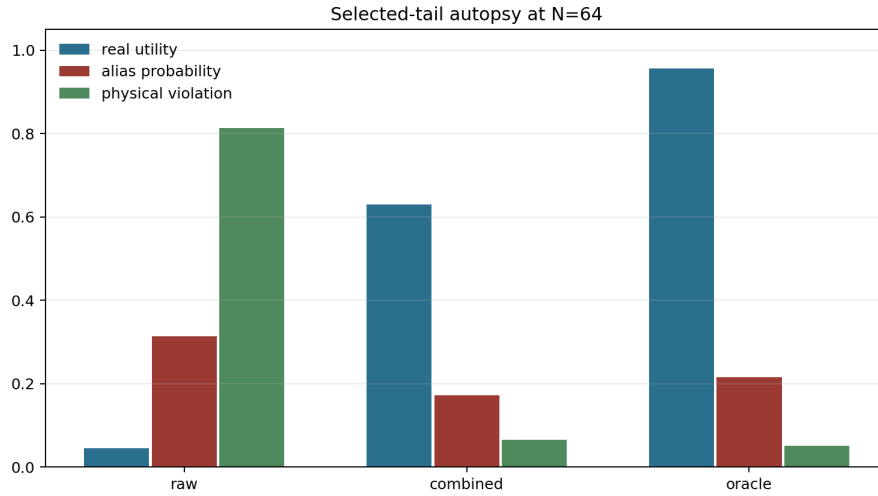
Figure 14: V3 tail autopsy. Raw high-budget selection chooses alias-heavy candidates; combined repair shifts the selected tail toward valid futures; oracle selects the highest real utility.
